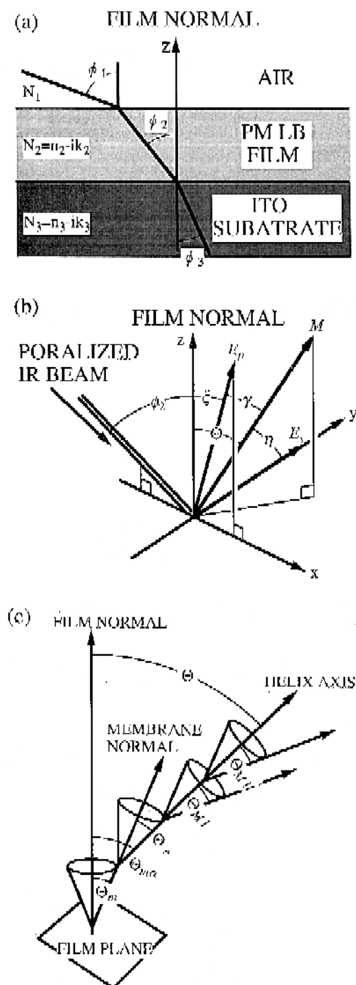
Fig. 3. (a) Reflection-absorbance at a three-phase (i.e., air, PM film, and ITO substrate) plane-bounded system. Here, N_1 , N_2 (= n_2 - i k_2) , and N_3 (= n_3 - i k_3) are the reflective indices of air, a PM LB film, and ITO, respectively. (b) Geometry for the electric vectors, E_p and E_s , of the incident polarized IR beam, and the averaged vector of transition moment, M , originating in amide groups of polypeptides of BR molecules at the interface of a PM film and ITO substrate. Here, \eta , \gamma , \xi , \Theta , and \phi are the angles. (c) Geometry of the four nested axially symmetric cones utilized for data analysis of the polarized IR spectra of an oriented PM film.
